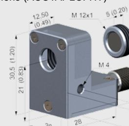
Air purge collar with integrated CF-lens (ACCTAPLCFHT)
