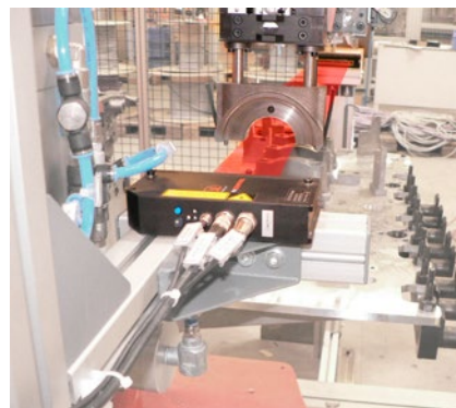
Bearing shell detection in automotive manufacturing
