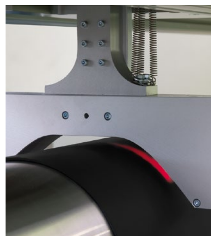
Thickness measurement of flat plastic film and rubber strips
