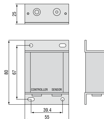
CP6001 capacitive pre-amplifier
