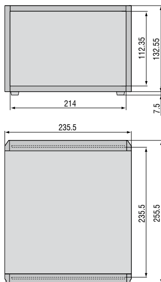
Controller DT6530C 2-channel rack
